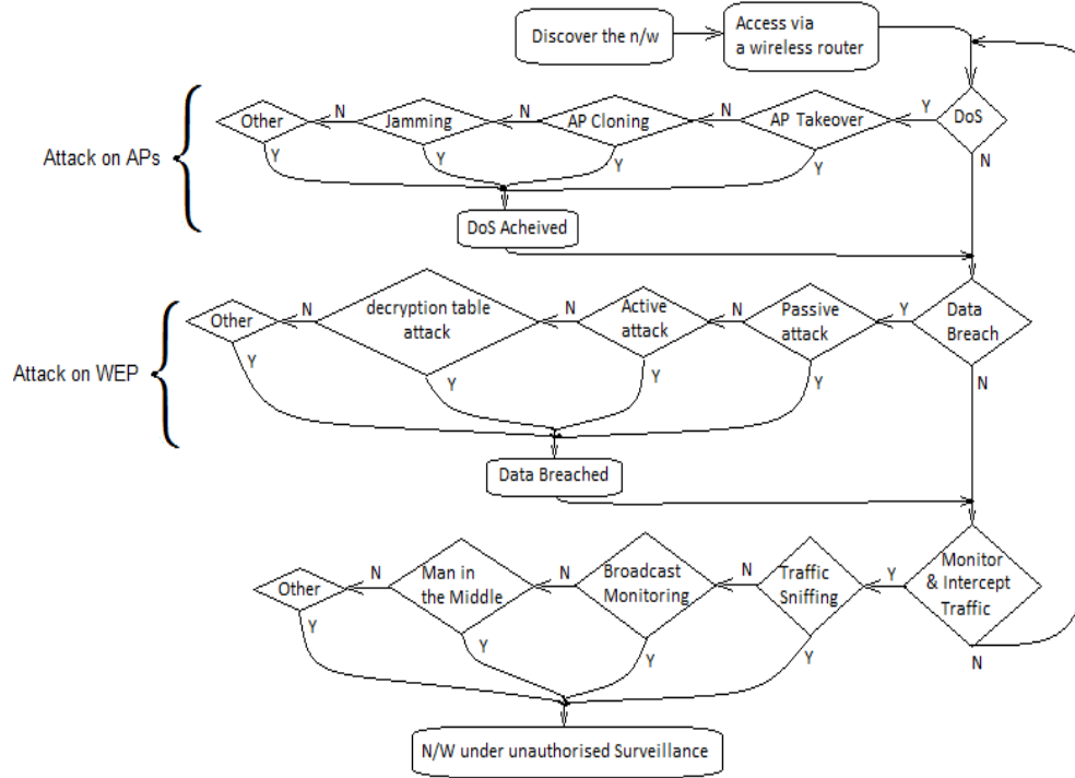
Fig. 3. Wireless Network Attack Tree.
